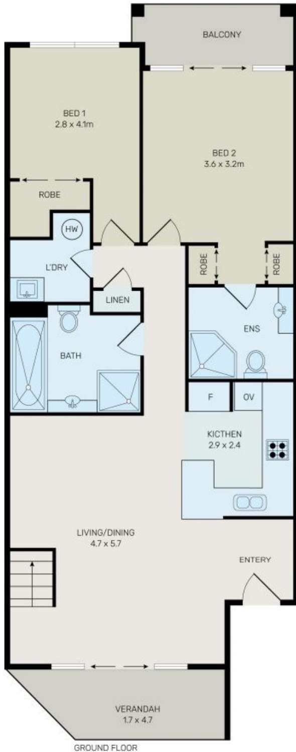
GROUND FLOOR
